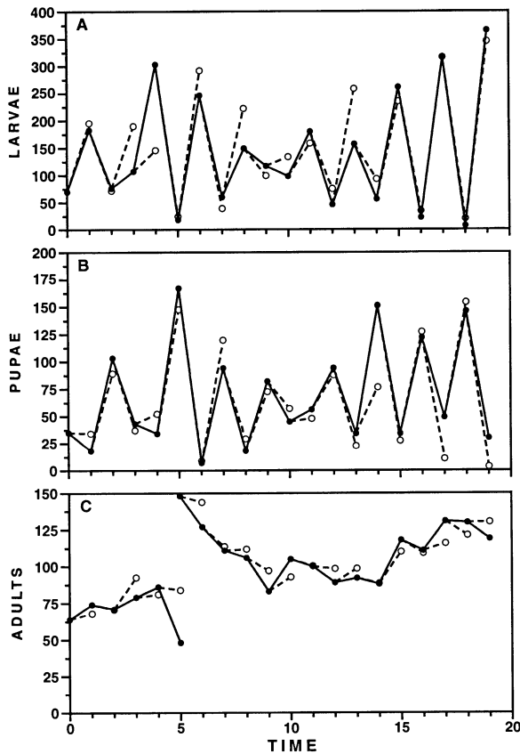
FIG. 14. Time series data (●) and one-step forecasts (○) for replicate B of Desharnais and Liu (1987) where 100 adults were added at t = 5 . Solid lines connect the observed census data. The one-step forecasts (dashed-line projections) are based on the parameter estimates obtained from the control cultures.
