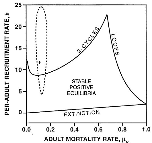
FIG. 3. Stability boundaries for the LPA model (Eqs. 1–3) for parameter values based on the experimental data (Table 1, all). The asterisk locates the estimated values of b = 11.68 and \mu_a = 0.1108 . The elongated closed curve (---) represents a 95% joint confidence region for b and \mu_a based on the profile likelihood.
