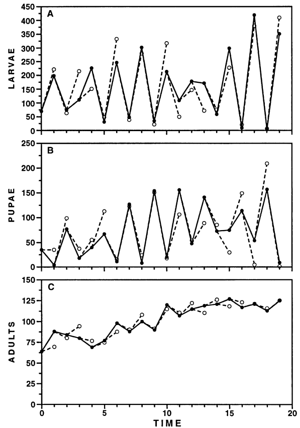
FIG. 8. Time series data (●) and one-step forecasts (○) for control replicate B of Desharnais and Liu (1987). Solid lines connect the observed census data. Dashed lines connect the observed numbers at time t with the forecast at time t + 1 .
