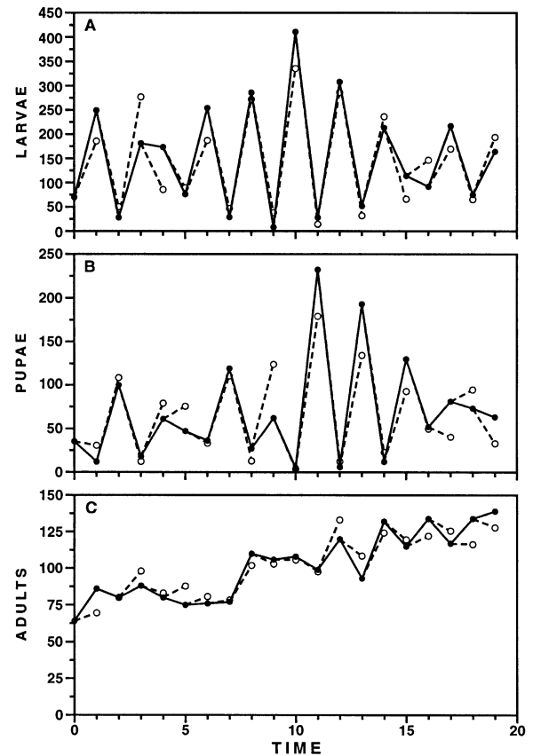
FIG. 10. Time series data (●) and one-step forecasts (○) for control replicate D of Desharnais and Liu (1987). Solid lines connect the observed census data. Dashed lines connect the observed numbers at time t with the forecast at time t + 1 .
