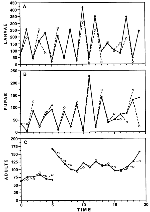
FIG. 15. Time series data (●) and one-step forecasts (○) for replicate C of Desharnais and Liu (1987) where 100 adults were added at t = 5 . Solid lines connect the observed census data. The one-step forecasts (dashed-line projections) are based on the parameter estimates obtained from the control cultures.
