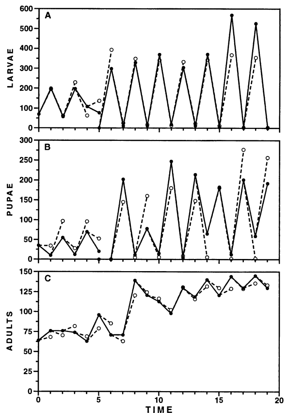
FIG. 19. Time series data (●) and one-step forecasts (○) for replicate A of Desharnais and Liu (1987) where all immatures were removed at t = 5 . Solid lines connect the observed census data. The one-step forecasts (dashed-line projections) are based on the parameter estimates obtained from the control cultures.
