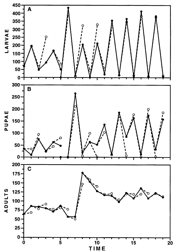
FIG. 21. Time series data (●) and one-step forecasts (○) for replicate C of Desharnais and Liu (1987) where all immatures were removed at t = 5 . Solid lines connect the observed census data. The one-step forecasts (dashed-line projections) are based on the parameter estimates obtained from the control cultures.
