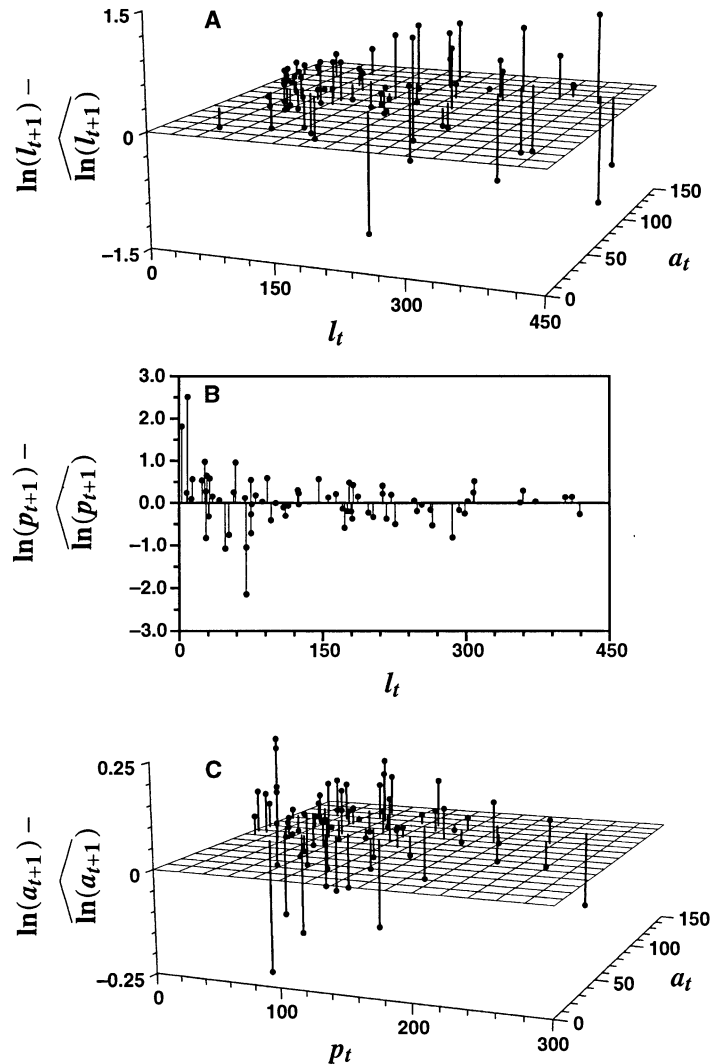
FIG. 12. Residual plots for the data from the four control replicates of Desharnais and Liu (1987). Deviations between the logarithms of the observed and predicted numbers of (A) larvae at time t + 1 as a function of the number of larvae and adults at time t , (B) pupae at time t + 1 as a function of the number of larvae at time t , and (C) adults at time t + 1 as a function of the number of pupae and adults at time t .
